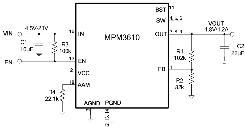
Figure 11: V_{OUT}=1.8V , I_{OUT}=1.2A
