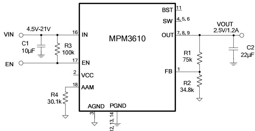
Figure 9: V_{OUT}=3.3V , I_{OUT}=1.2A
