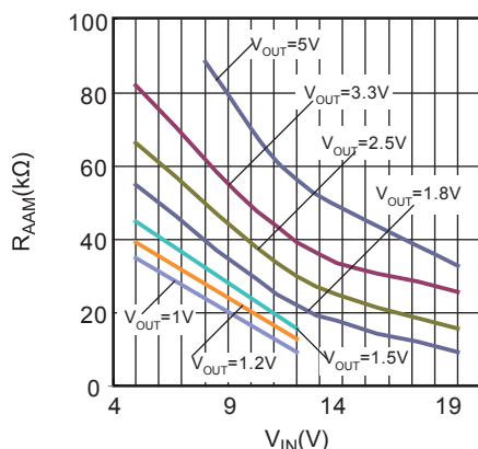
Figure 7: AAM Resistor Selection
