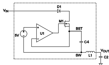
Figure 4: Internal Bootstrap Charging Circuit
