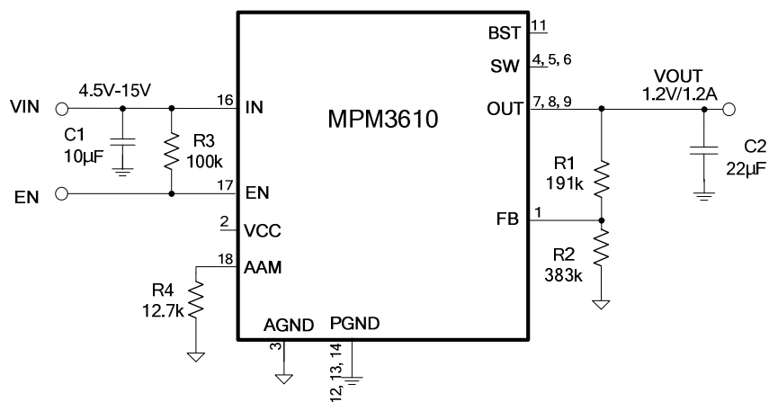
Figure 12: V_{OUT}=1.2V , I_{OUT}=1.2A
