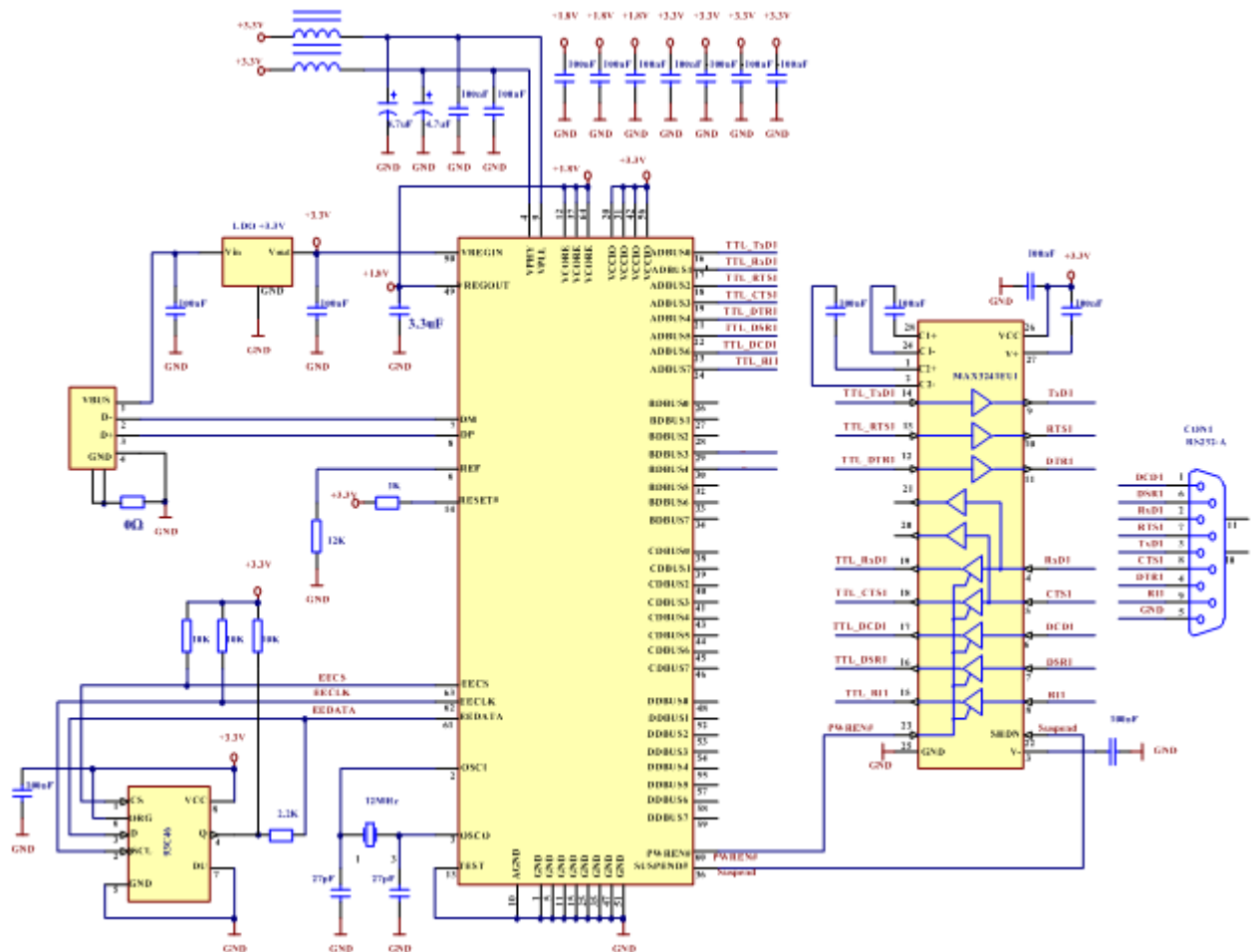
Figure 4.1 RS232 Configuration
